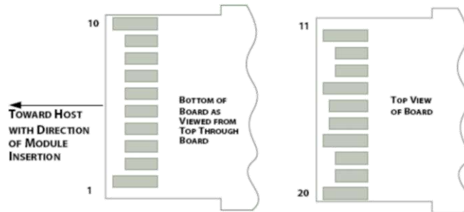
Figure 6 : Module Contact Assignment
