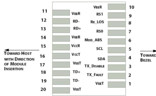
Figure 5: Interface to Host PCB
