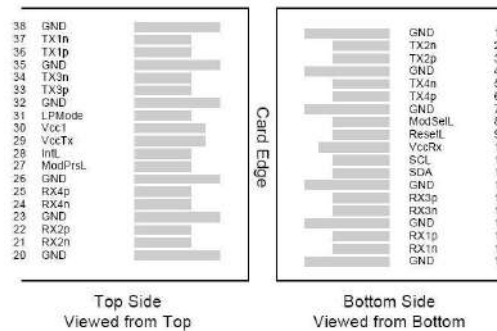
Module Interface to Host
